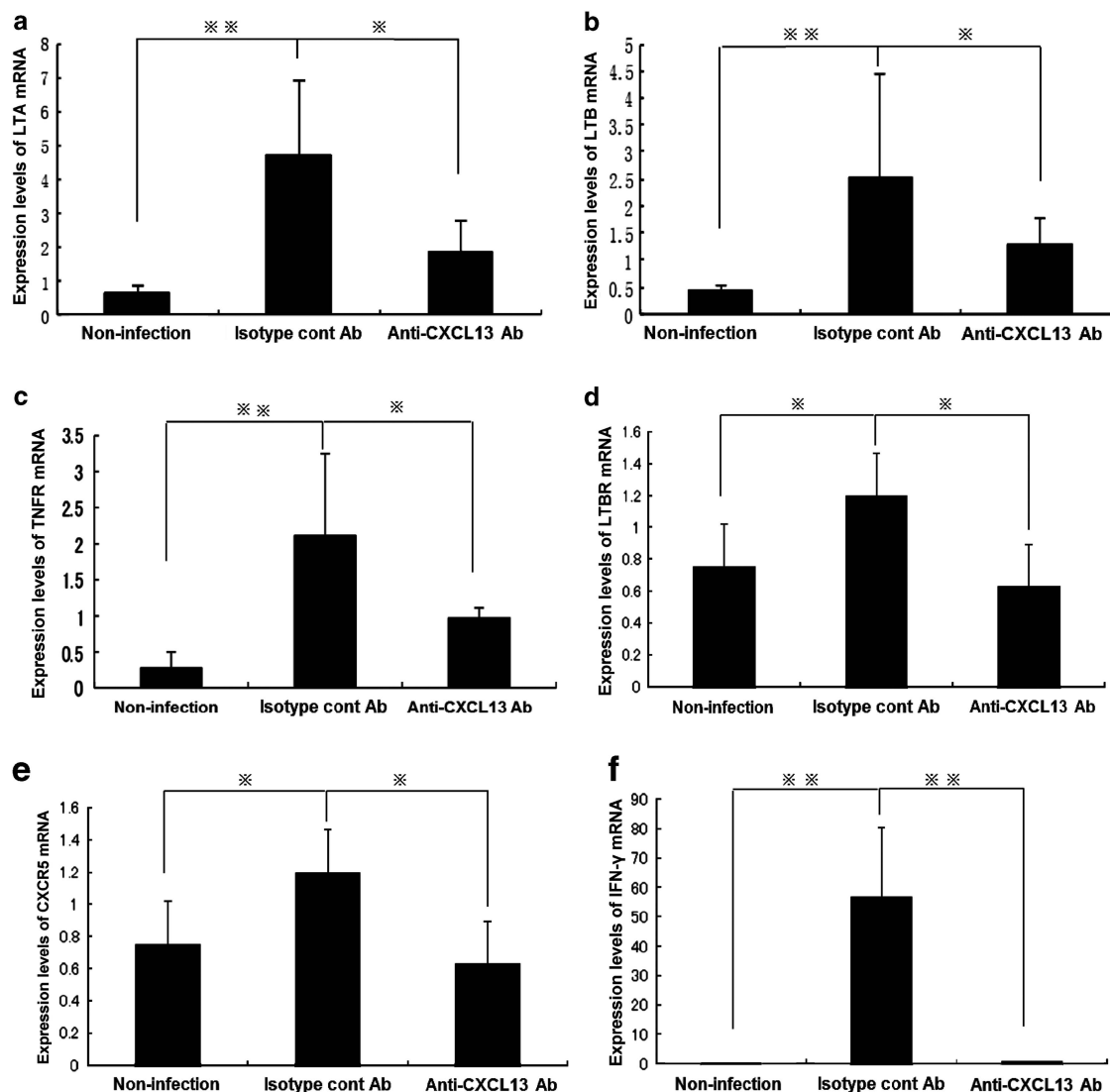
Figure 5 The expression level of lymphoid follicles associated genes in the stomachs of H. suis -infected mice after anti-CXCL13 antibody treatment. The C57BL/6J mice (each n = 10 ) were treated with anti-CXCL13 antibody or the isotype control antibody weekly for 3 months starting 1 week after H. suis infection as described in Methods. The mRNA expression levels of lymphotoxin A (a), lymphotoxin B (b), CXCR5 (c), tumor necrosis factor receptor 1 (TNFR1) (d), lymphotoxin B receptor (LTBR) (e), and interferon- \gamma (IFN \gamma ) (f) in the gastric mucosa were determined by real-time quantitative PCR. The mRNA expression levels were normalized to those of \beta -actin as an internal standard. Data are representative of at least three independent experiments for each mouse and shown as the mean \pm s.d. ( n = 10 ). * P < 0.05 ; ** P < 0.01 according to the Student's t -test.
