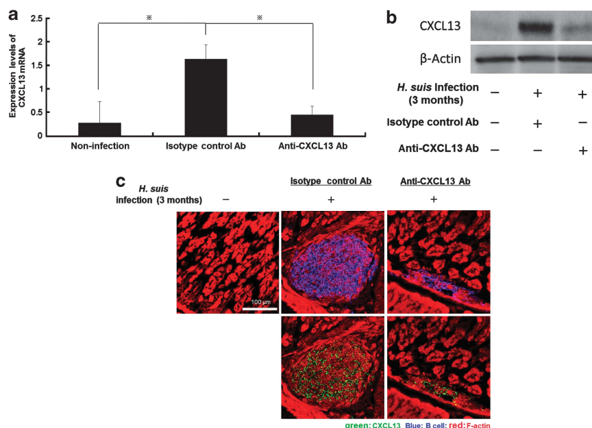
Figure 2 Suppression of expression of CXCL13 in the stomachs of H. suis -infected mice after anti-CXCL13 antibody treatment. The C57BL/6J mice (each n = 10 ) were treated with anti-CXCL13 antibody or the isotype control antibody weekly for 3 months starting 1 week after H. suis infection as described in Methods. (a) The mRNA expression levels of CXCL13 in the gastric mucosa were determined by real-time quantitative PCR. The mRNA expression levels were normalized to those of \beta -actin as an internal standard. Data are representative of at least three independent experiments for each mouse and shown as the mean \pm s.d. ( n = 10 ). *P < 0.05 according to the Student's t -test. (b) The proteins were obtained from the stomach of the anti-CXCL13 antibody or isotype control antibody-treated mice with H. suis infection, and were subjected to immunoblotting using anti-CXCL13 antibody or anti- \beta -actin antibody. Data are representative of at least three independent experiments for each mouse ( n = 10 ) and typical images are shown. (c) Immunohistological examination of the gastric mucosa was performed by confocal laser scanning microscopy, and the selected serial sections were stained with anti-CXCL13 antibody in a blind manner. Green: CXCL13; blue: B220; and red: F-actin. Original magnification \times 200 . Bar = 100 \mu m. Data are representative of at least three independent experiments for each mouse ( n = 10 ) and typical images are shown.
